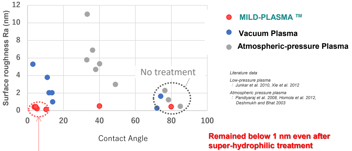
Water contact angle and surface roughness of PET films after plasma treatment
